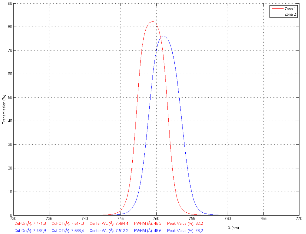
Bandas Moleculares, 7500/50
